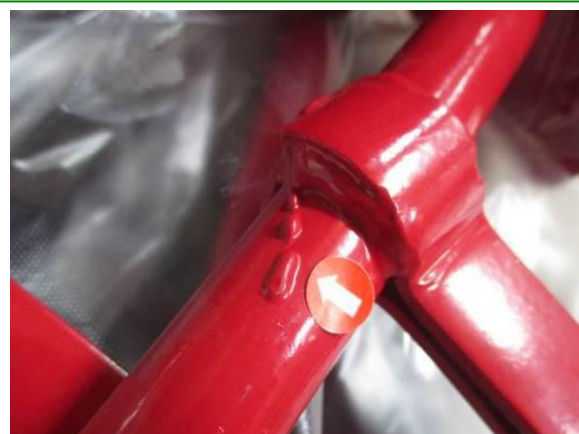
71). Minor defect – slag attached on body
